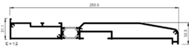
Cill 250mm
