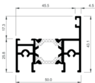
Central sash
