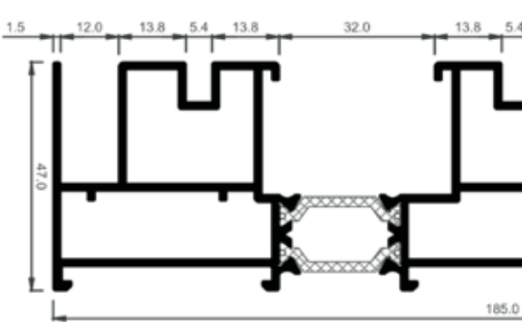
Three rail
