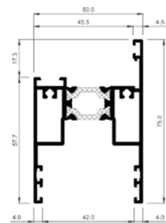
Perimeter sash
