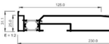
Cill 230mm
